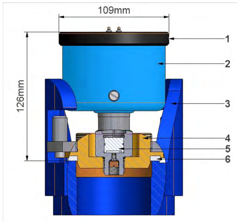
Figure 10: ESS3 water housing with bayonet adapter
