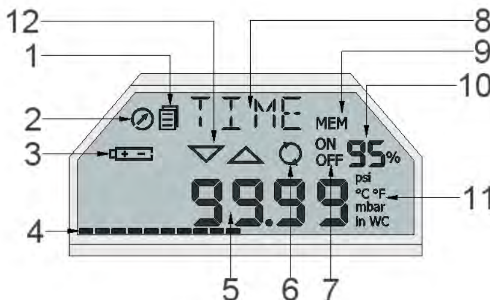
Figure 5: ESS3 display indications
